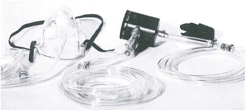
Figure 11 - PreciseFlow ® Oxygen Conservers Breathing Station Kit (with Dual Lumen Cannula and Standard Dual Supply Mask Shown)
