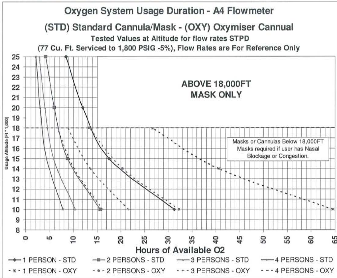
Figure 25 - A4 Flowmeter (Oxymizer and STD Scales)
