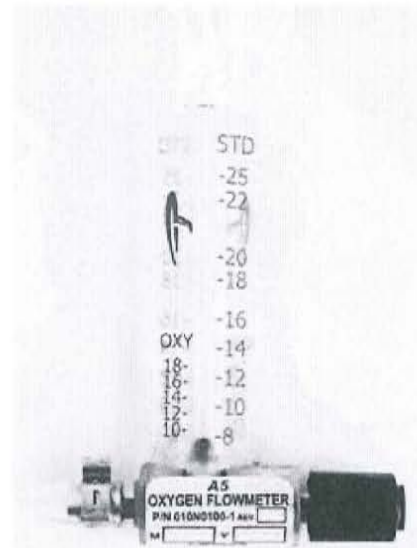
Figure 9 – A5 Constant Flow Oxygen Flowmeter
