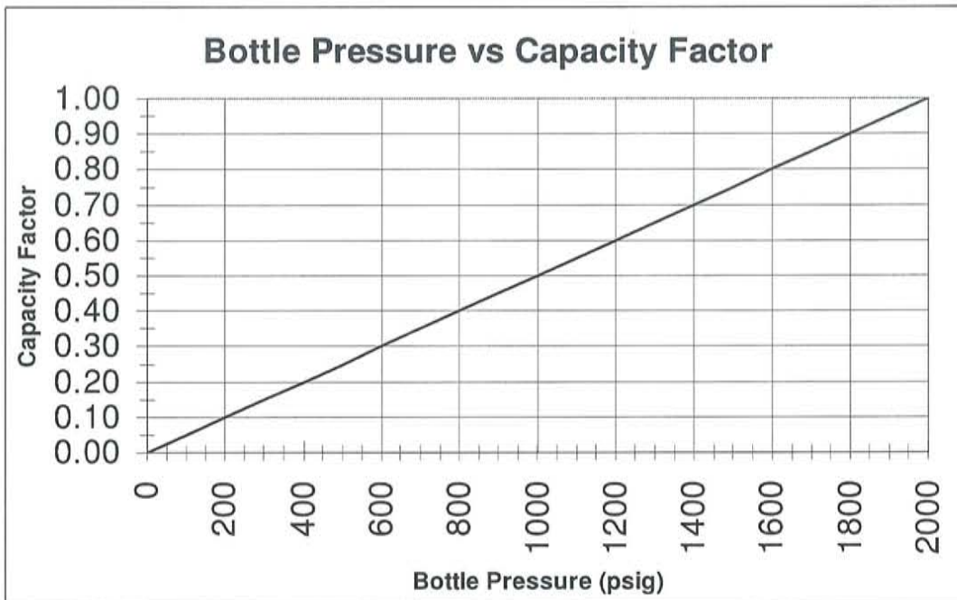
Figure 24 - Bottle Pressure/Capacity Factor Graph
