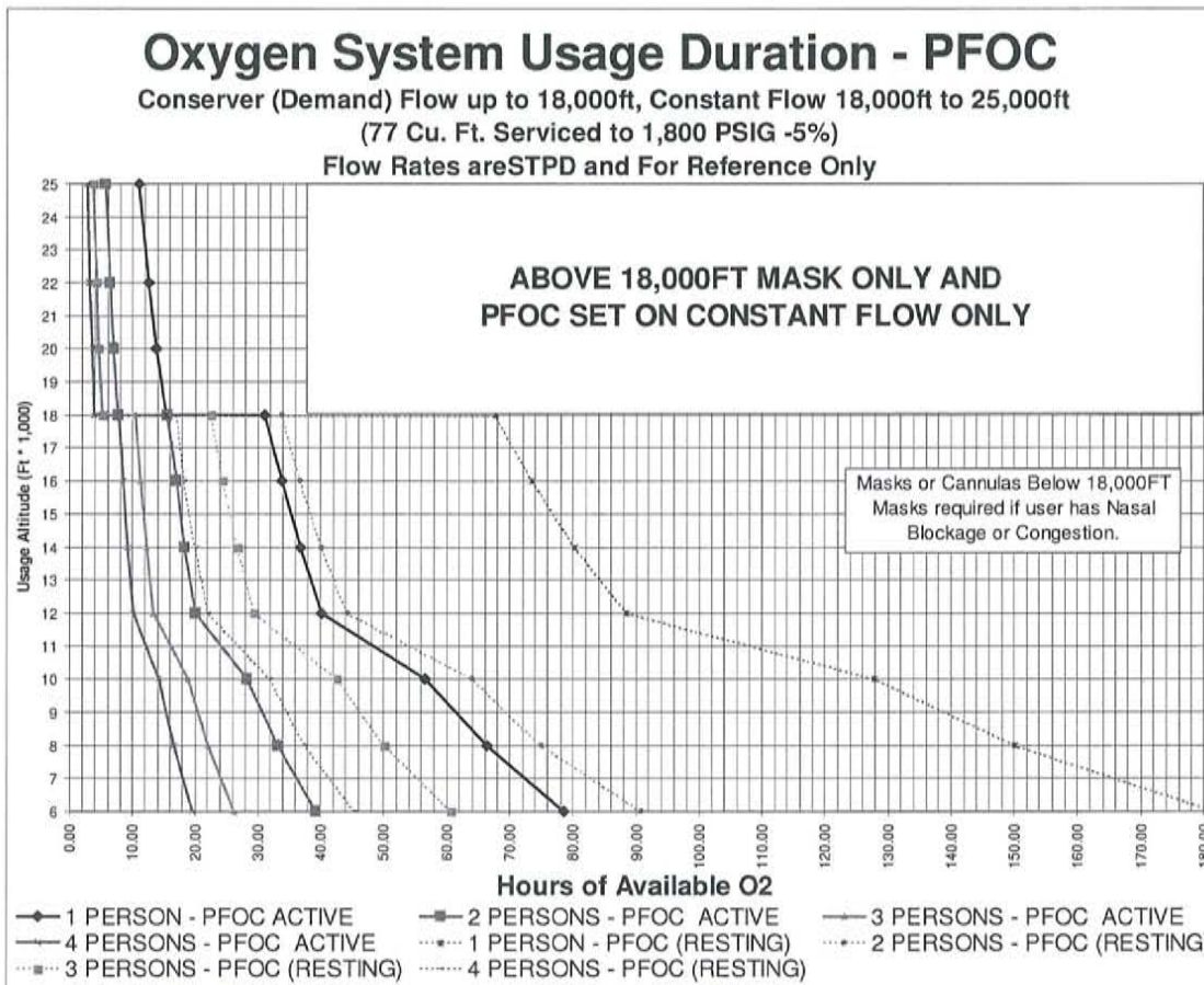
Figure 27 - PreciseFlow Oxygen Conserver
