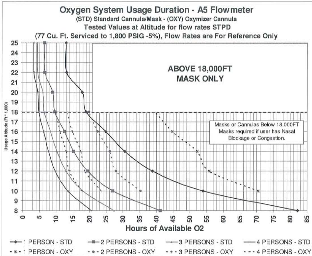
Figure 26 - A5 Flowmeter (Oxymizer and Standard Scales)
